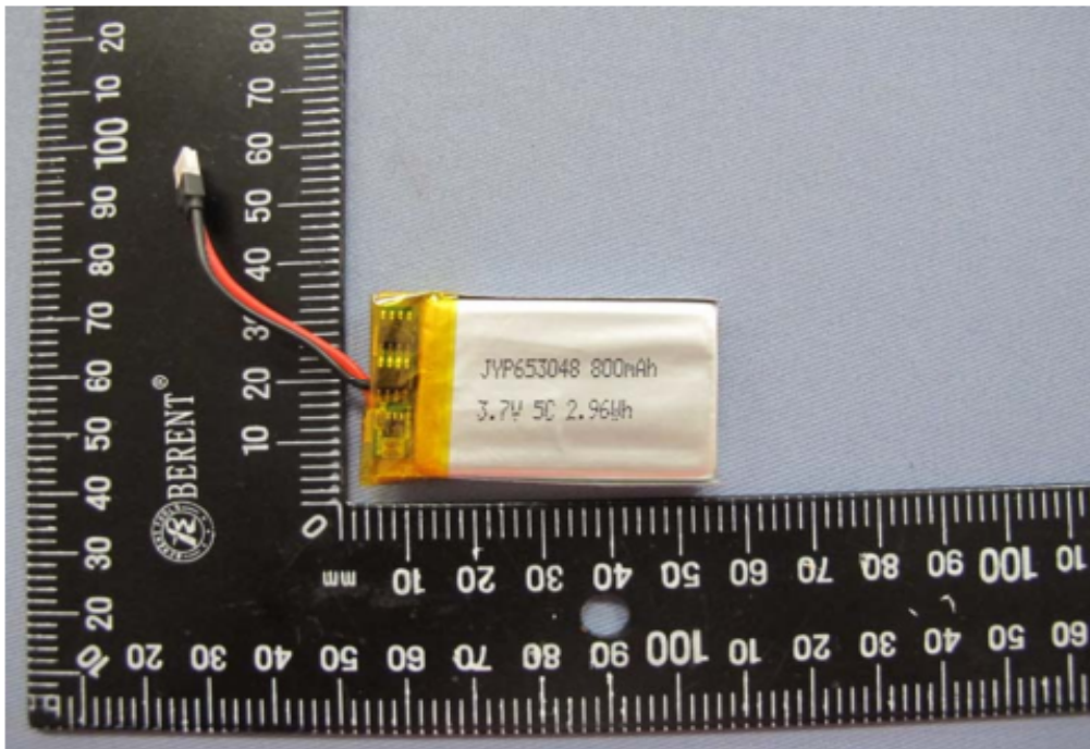
Fig.1 Overall view I of battery
