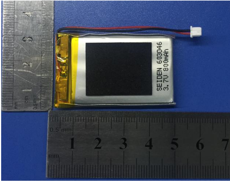
Figure 2 Bottom view of battery
